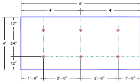
6 FASTENERS PER 4'-0" X 8'-0" BOARD
