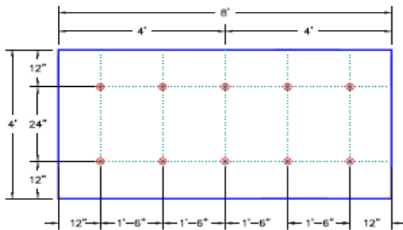
10 FASTENERS PER 4'-0" X 8'-0" BOARD
