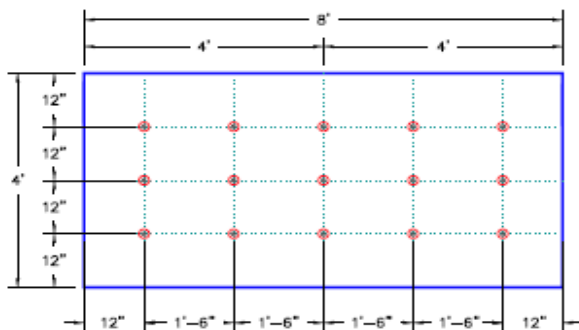
15 FASTENERS PER 4'-0" X 8'-0" BOARD
