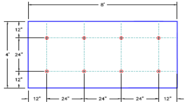
8 FASTENERS PER 4'-0" X 8'-0" BOARD
