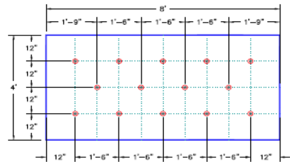
14 FASTENERS PER 4'-0" X 8'-0" BOARD
