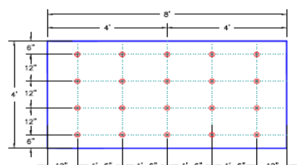
20 FASTENERS PER 4'-0" X 8'-0" BOARD
